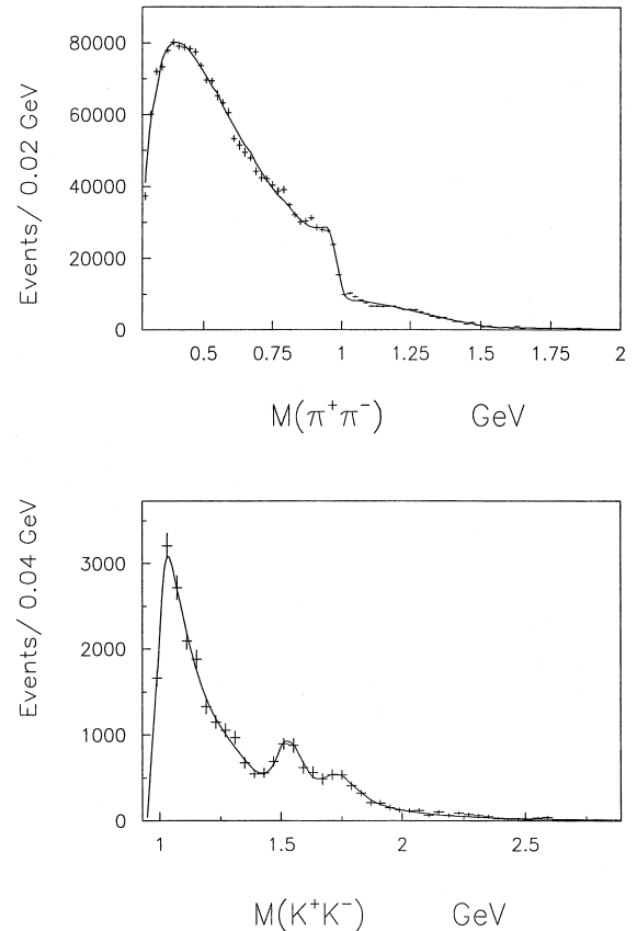
Fig. 2. A coupled channel fit to the \pi^+ \pi^- and K^+ K^- S-wave distributions.
