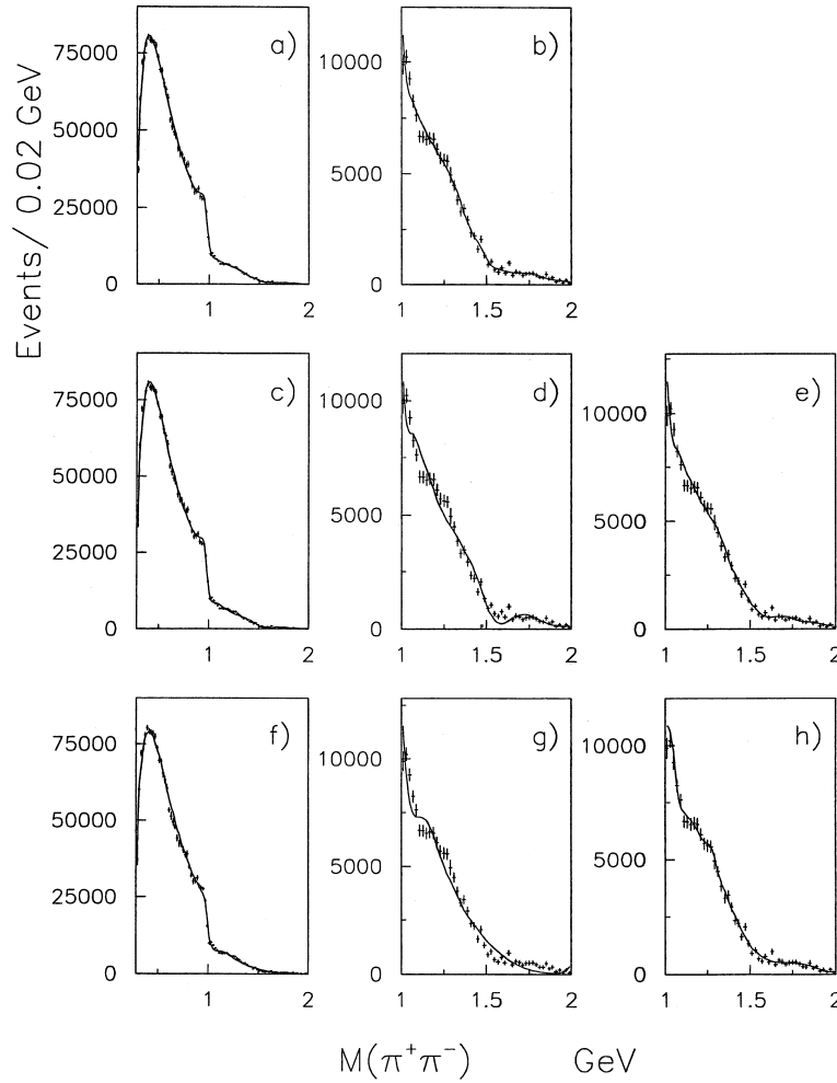
Fig. 1. The \pi^+ \pi^- mass spectrum with a) and b) fit using interfering Breit-Wigners. Fit using the T-Matrix parameterisation c) and d) the original fit and e) including two extra poles. Fit using the K-Matrix parameterisation f) and g) the original fit and h) including another two poles.
