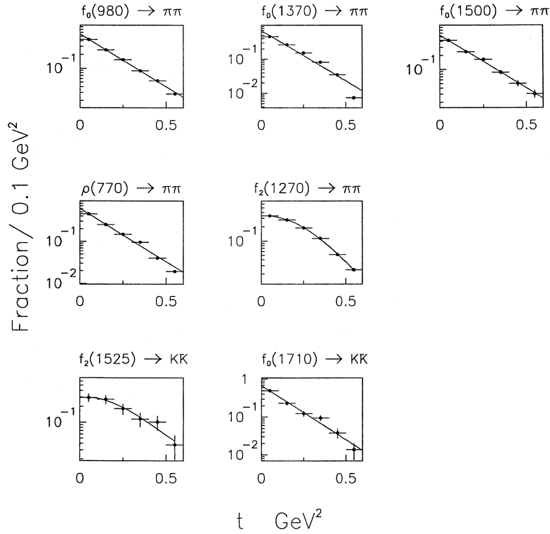
Fig. 5. The four momentum transfer squared ( |t| ) from one of the proton vertices for the resonances observed in the \pi^+\pi^- and K^+K^- channels.
