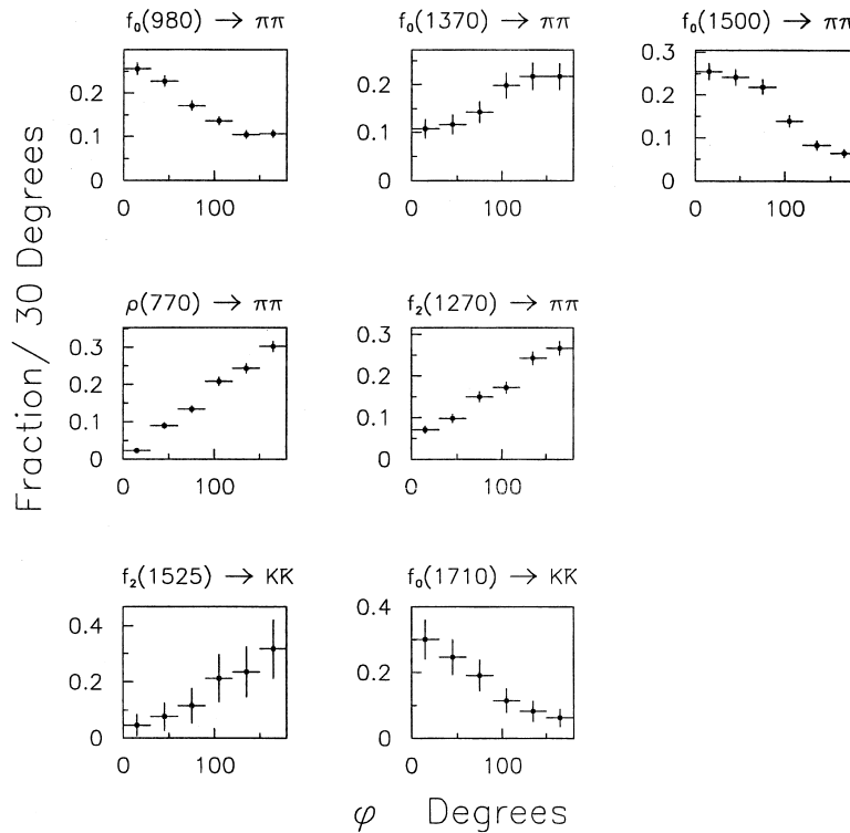
Fig. 4. The \phi distributions of the resonances observed in the \pi^+ \pi^- and K^+ K^- channels.
