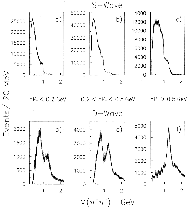
Fig. 3. The \pi^+\pi^- S-wave and D-wave in three dP_T intervals.
